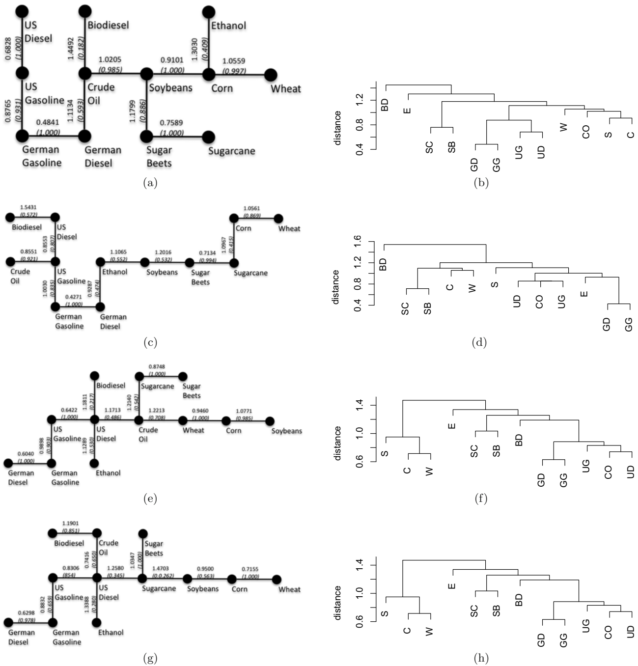
Fig. 4. Fuels. Notation and ordering holds from Figure 2.
