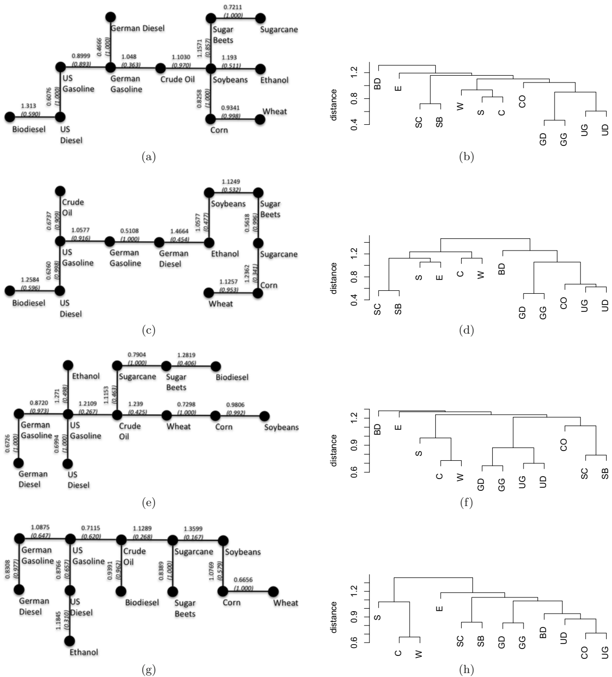
Fig. 2. Crude oil. Results are shown for the high crude oil prices (a)–(d) and for low crude oil prices (e)–(h) with MSTs on the left (a,c,e,g) and HTs on the right (b,d,f,h). Weekly (a,b,e,f) and monthly (c,d,g,h) frequencies are shown.
