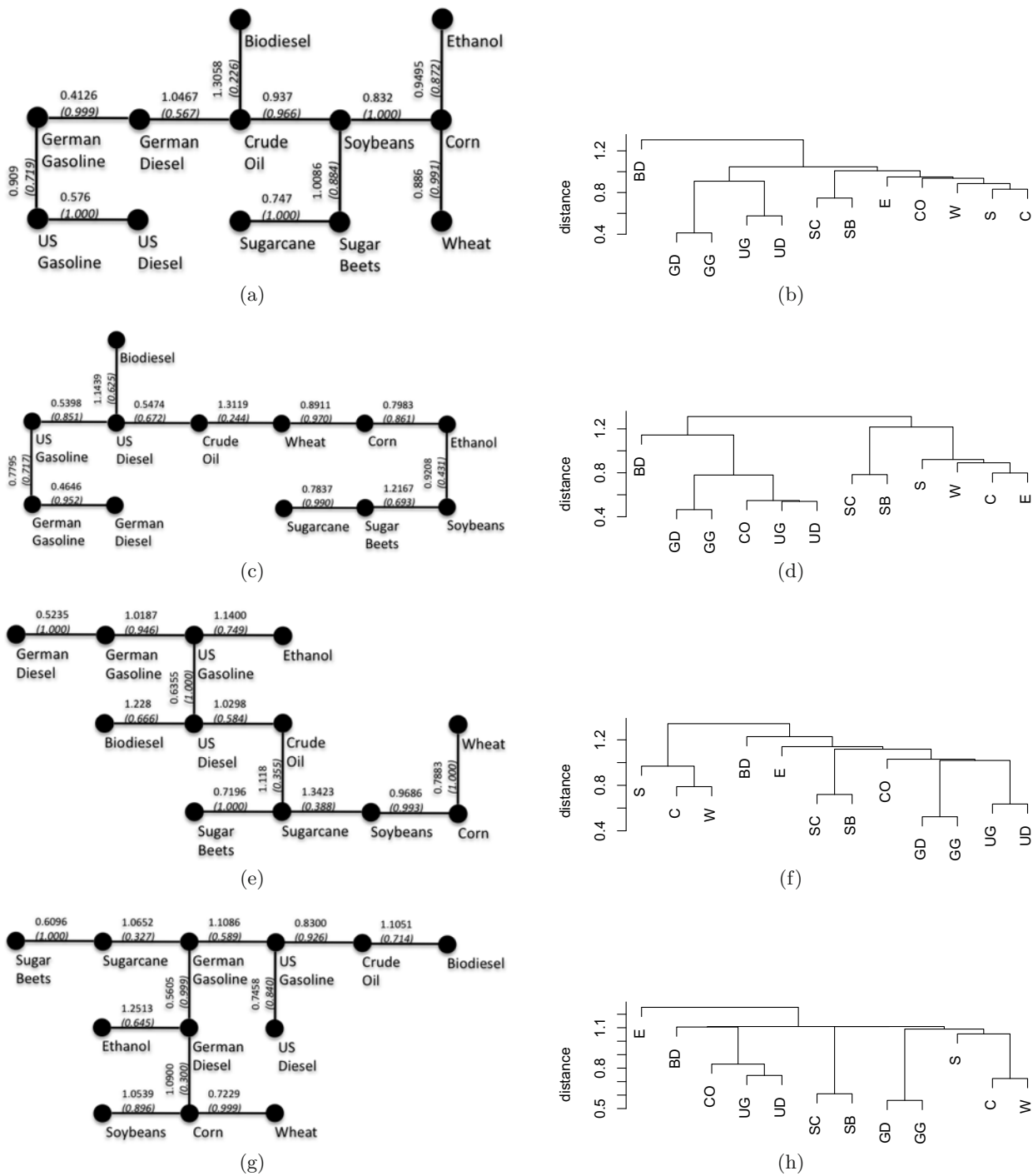
Fig. 3. Corn & wheat. Notation and ordering holds from Figure 2.
