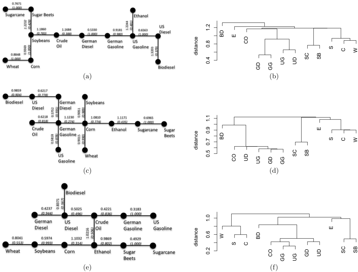
Fig. 1. Minimal spanning trees (first column) and hierarchical trees (second column) for network of returns and different frequencies (from the top – one week, one month and one quarter).
